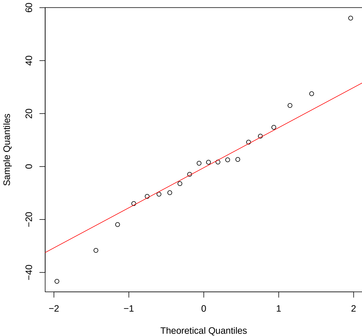
QQ plot residuals - >5 px
